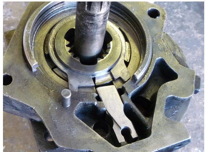
25. The pawl is installed with the machined relief at the lower left facing up. This will align the curve in the pawl with the hole in the casting. Note the direction of the angle at the top end of the pawl.
