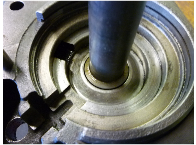
23. The blocking assembly is inserted into this recess. The pawl is inserted and actuates in the slot at lower left.
